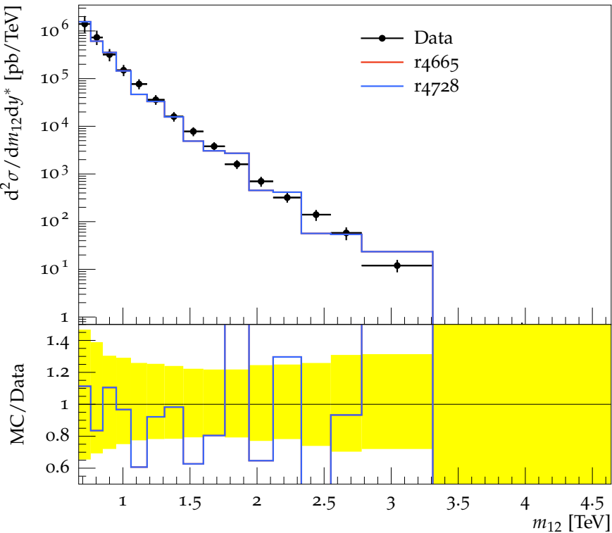
Dijet double-diff. x-section, anti- k_t 0.6 ( 2.5 \leq y^* < 3.0 )
