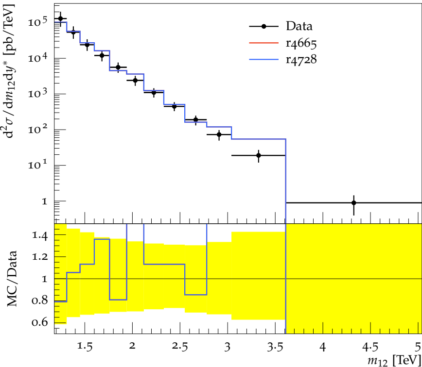
Dijet double-diff. x-section, anti- k_t 0.6 ( 3.0 \leq y^* < 3.5 )
