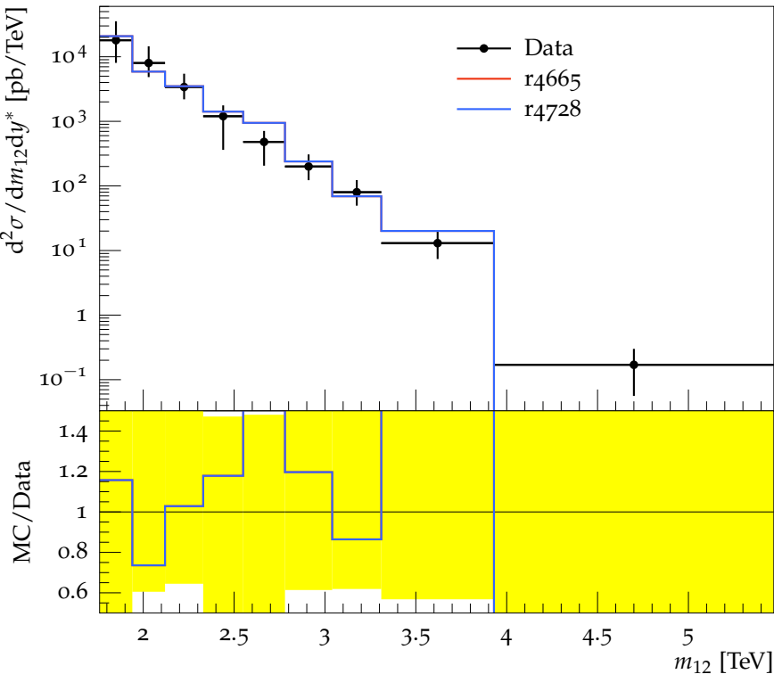
Dijet double-diff. x-section, anti- k_t 0.6 ( 3.5 \leq y^* < 4.0 )
