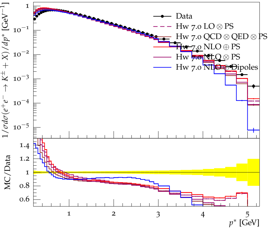
Spectrum for e^+e^- \rightarrow K^\pm + X including K_S and \Lambda decays
