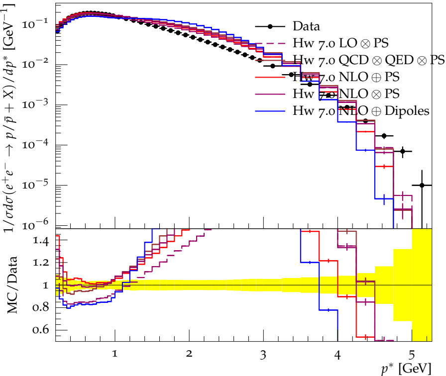
Spectrum for e^+e^- \rightarrow p/\bar{p} + X including K_S and \Lambda decays
