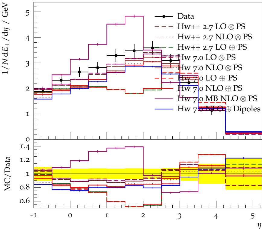
Transverse energy flow for \langle x \rangle = 0.01, \langle Q^2 \rangle = 253 \text{ GeV}^2
