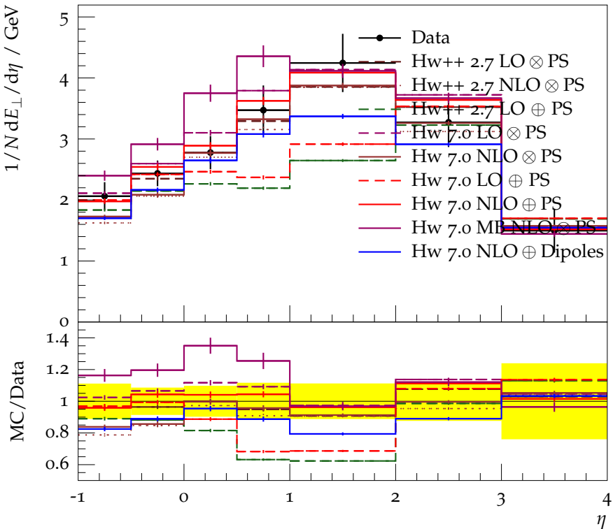
Transverse energy flow for \langle x \rangle = 0.11, \langle Q^2 \rangle = 2200 \text{ GeV}^2
