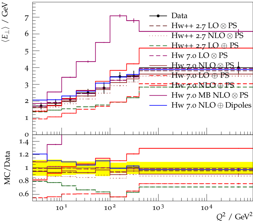
Average E_{\perp} in the forward region
