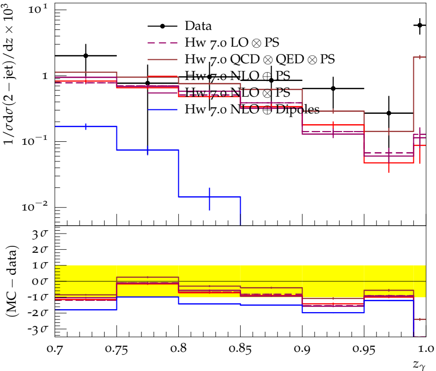
Photon Fragmentation in 2-jet events with y_{\text{cut}} = 0.01
