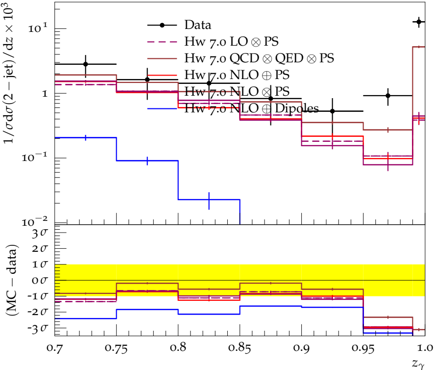
Photon Fragmentation in 2-jet events with y_{\text{cut}} = 0.06
