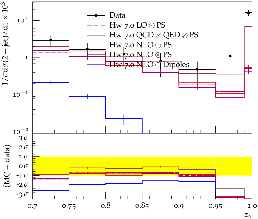
Photon Fragmentation in 2-jet events with y_{\text{cut}} = 0.1
