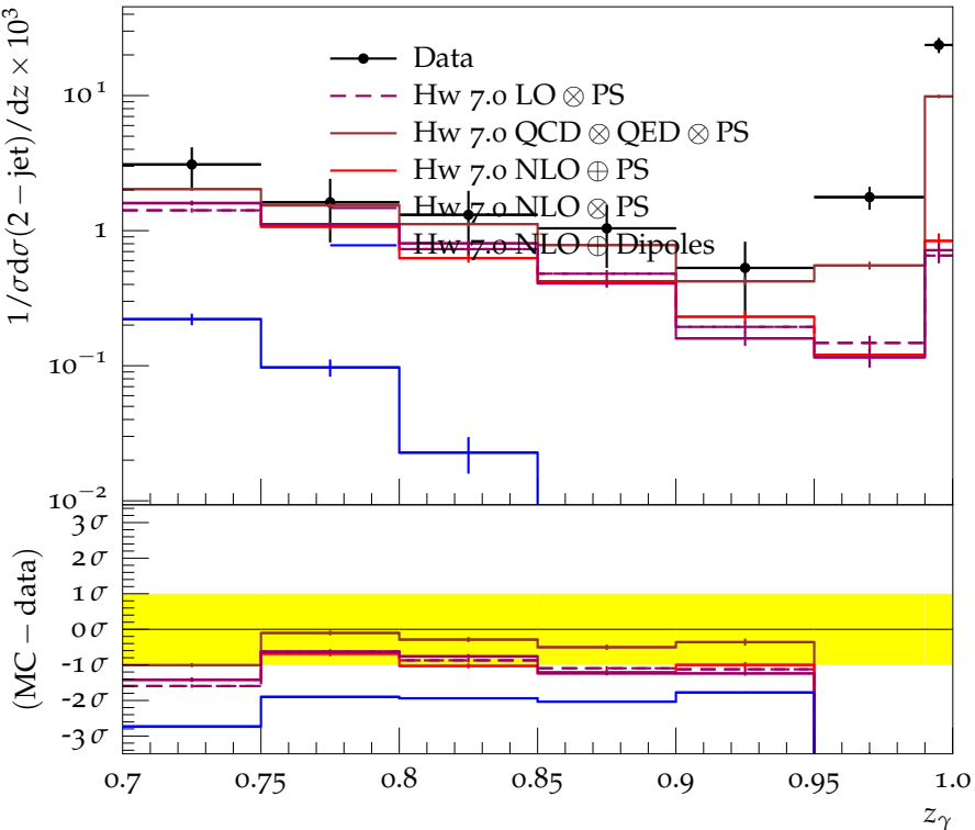
Photon Fragmentation in 2-jet events with y_{\text{cut}} = 0.33
