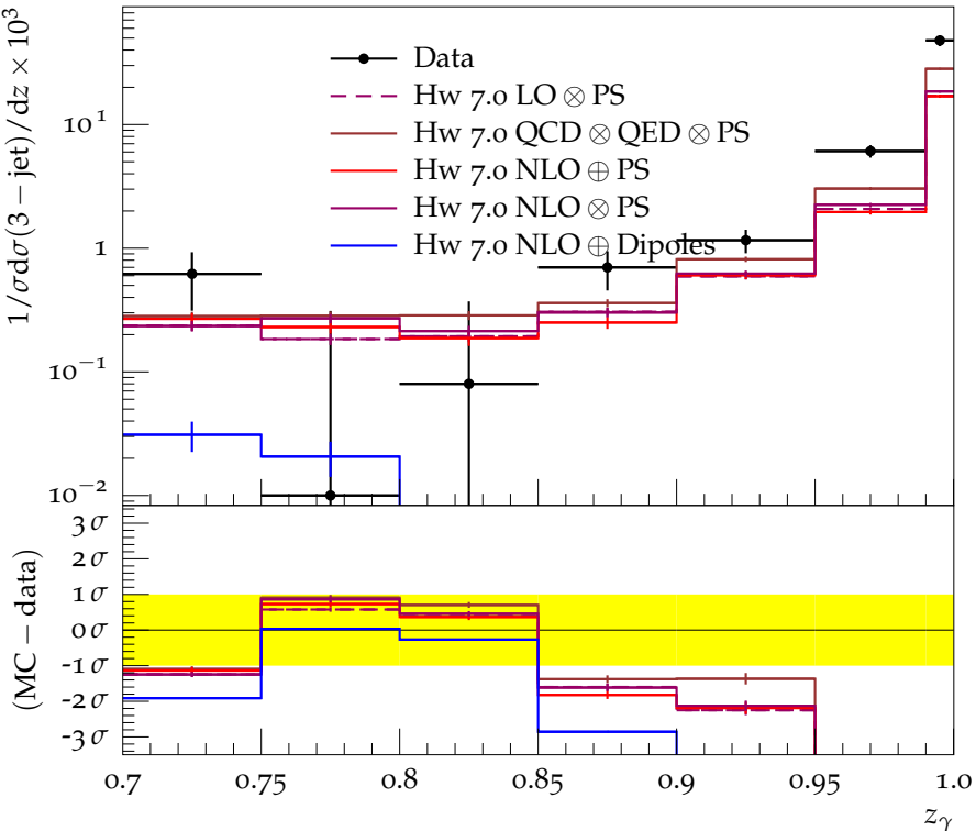
Photon Fragmentation in 3-jet events with y_{\text{cut}} = 0.06
