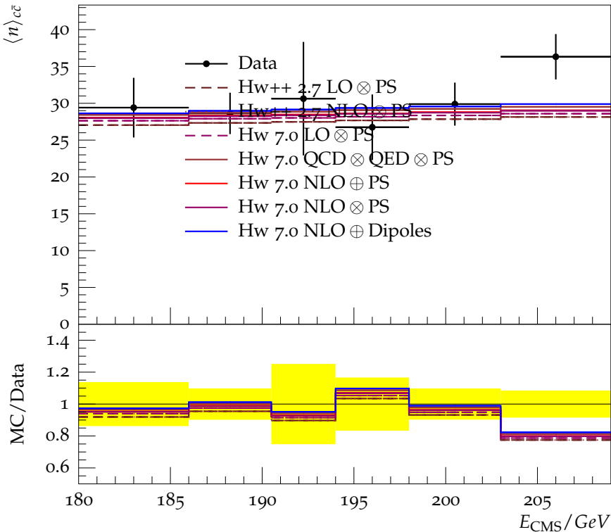
Charged multiplicity as a function of energy in c events
