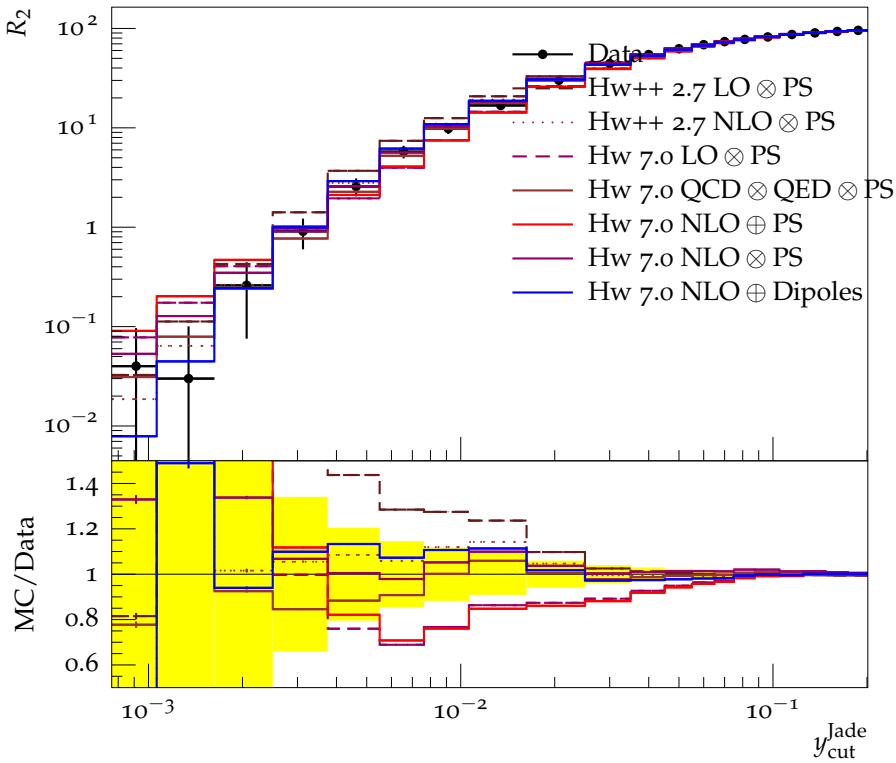
Integrated 2-jet rate with Jade algorithm (35 GeV)
