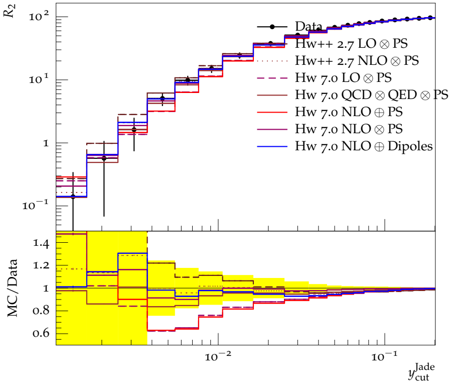
Integrated 2-jet rate with Jade algorithm (44 GeV)
