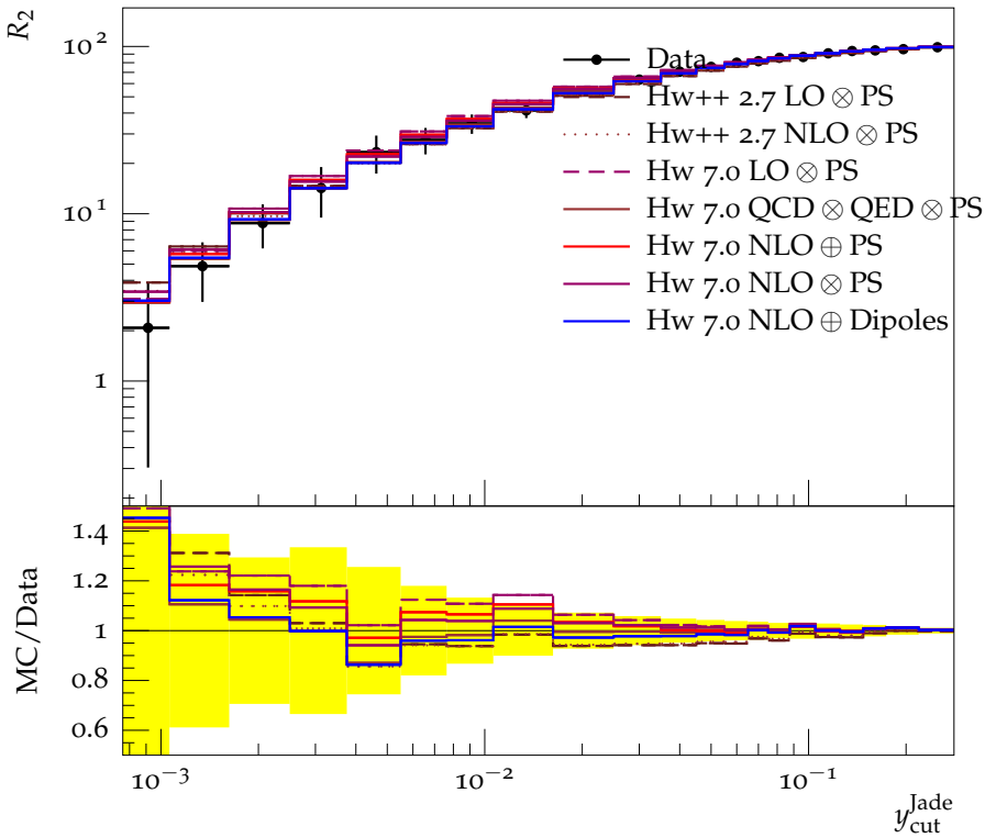
Integrated 2-jet rate with Jade algorithm (172 GeV)
