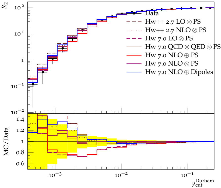
Integrated 2-jet rate with Durham algorithm (44 GeV)
