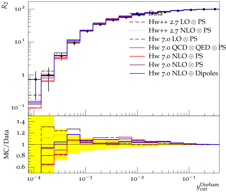
Integrated 2-jet rate with Durham algorithm (133 GeV)
