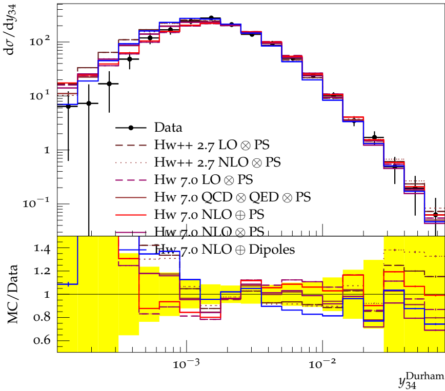
Differential 3-jet rate with Durham algorithm (44 GeV)
