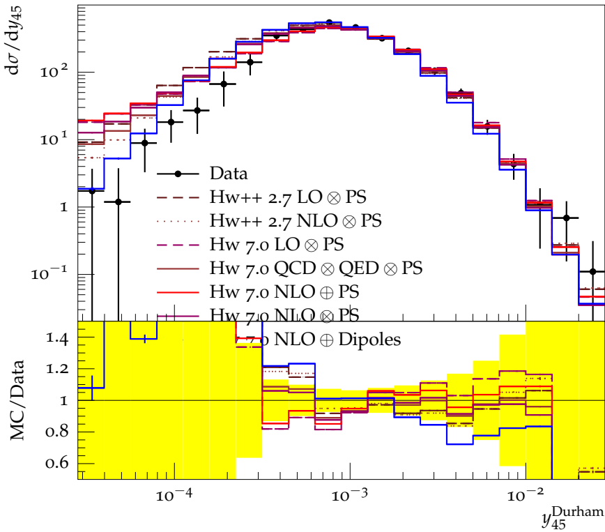
Differential 4-jet rate with Durham algorithm (44 GeV)
