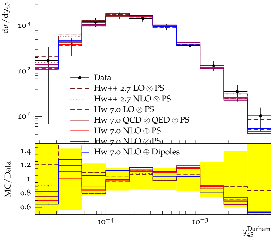
Differential 4-jet rate with Durham algorithm (133 GeV)
