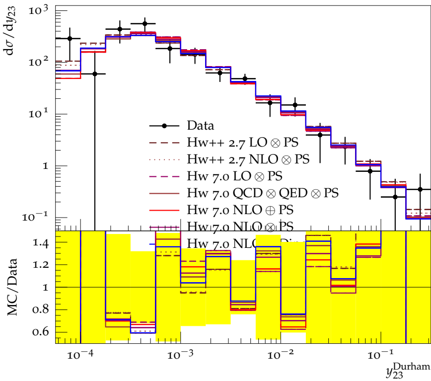
Differential 2-jet rate with Durham algorithm (172 GeV)
