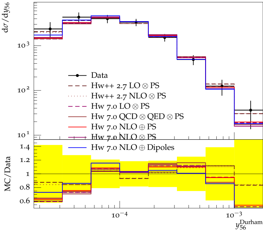
Differential 5-jet rate with Durham algorithm (172 GeV)
