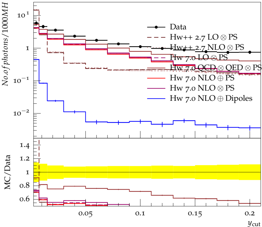
Number of photon vs y_{\text{cut}} , Jade
