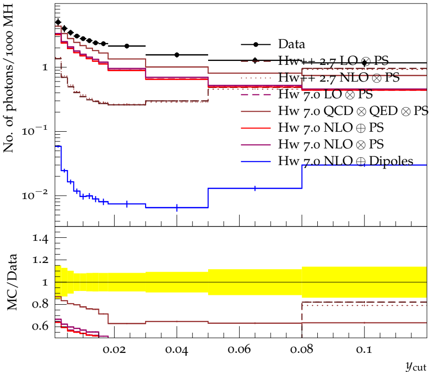
Number of photon vs y_{\text{cut}} , Durham
