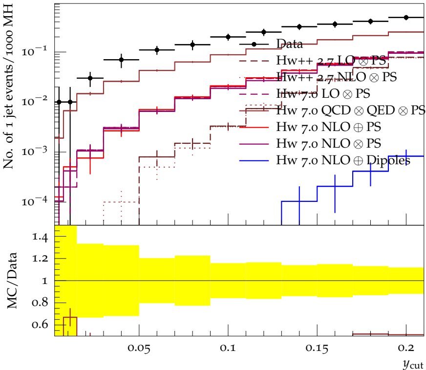
Number of 1 jet events vs y_{cut} , Jade
