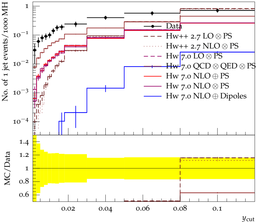
Number of 1 jet events vs y_{cut} , Durham
