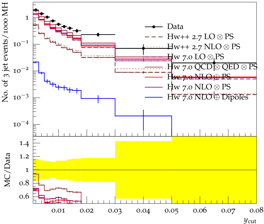
Number of 3 jet events vs y_{cut} , Durham
