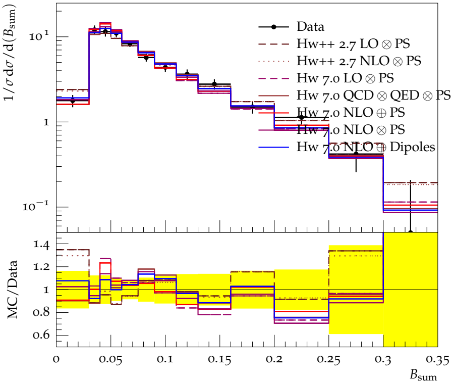
Total hemisphere broadening, B_{\text{sum}} , at 177 (161–183) GeV
