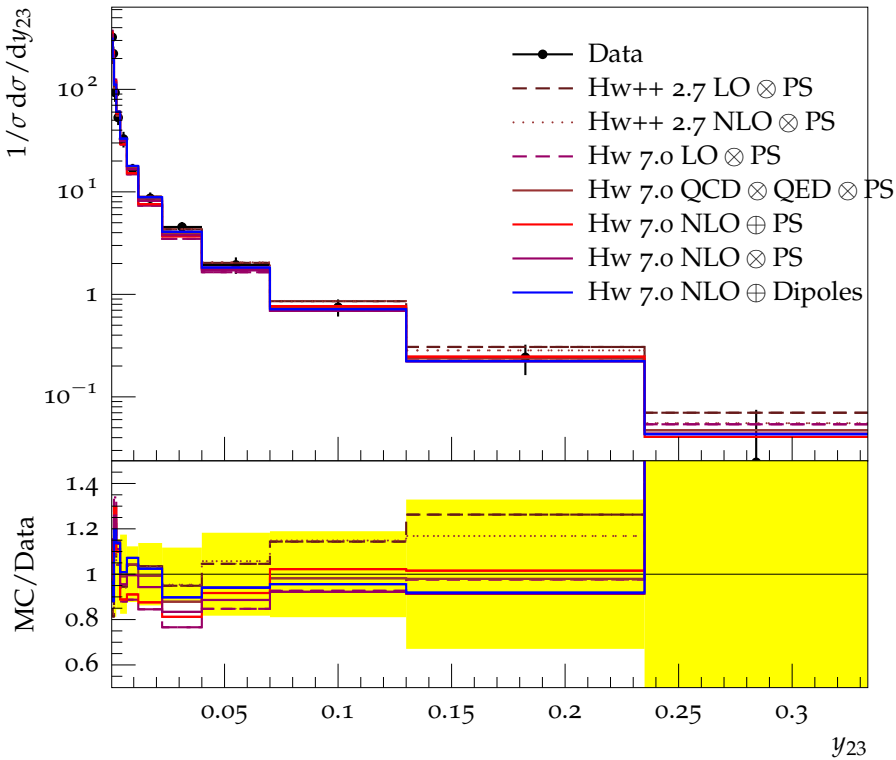
Durham jet 2 \rightarrow 3 transition parameter, y_{23} , at 177 (161–183) GeV
