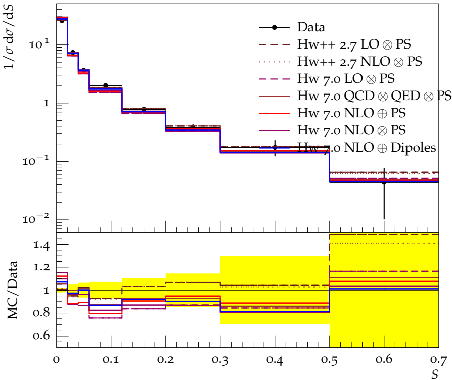
Sphericity, S , at 197 (189–209) GeV
