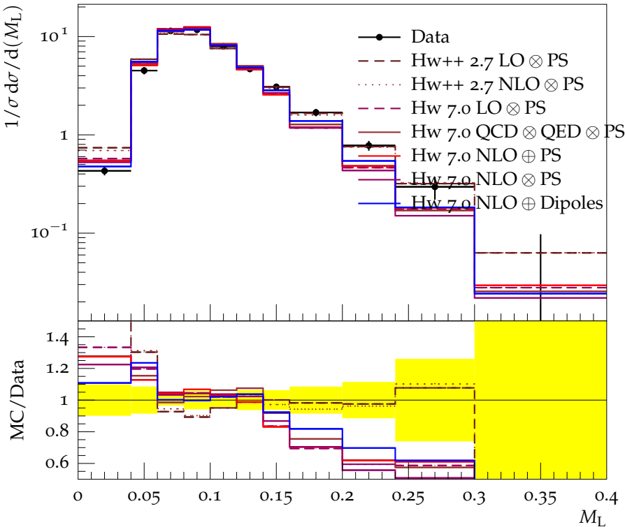
Light hemisphere mass, M_L , at 197 (189–209) GeV
