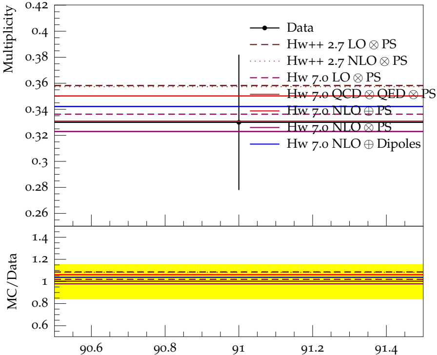
Mean B^+, B_d^0 multiplicity
