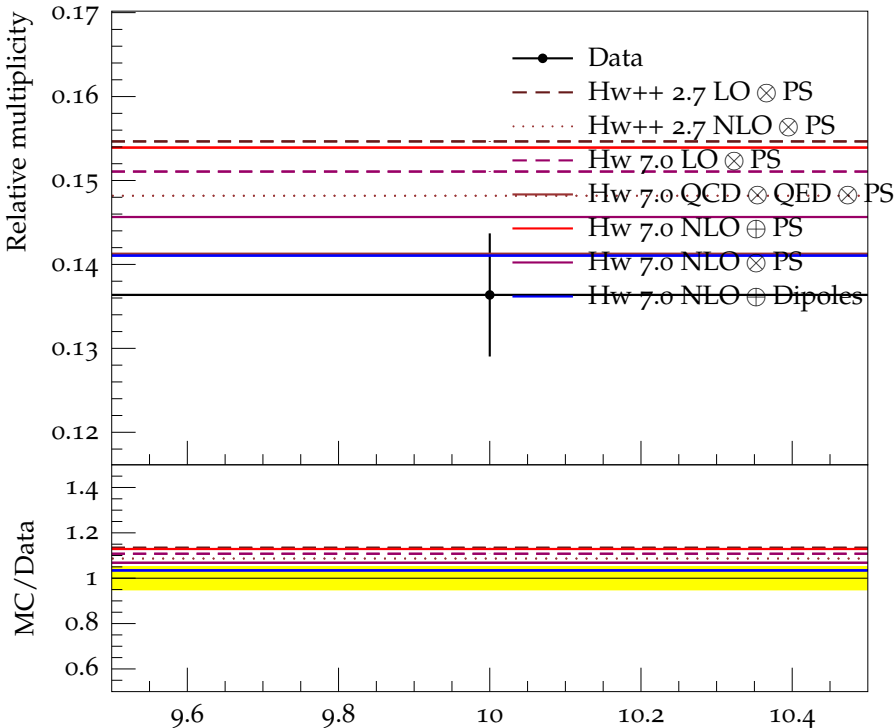
Ratio (w.r.t. \pi^\pm ) of mean K^+ multiplicity
