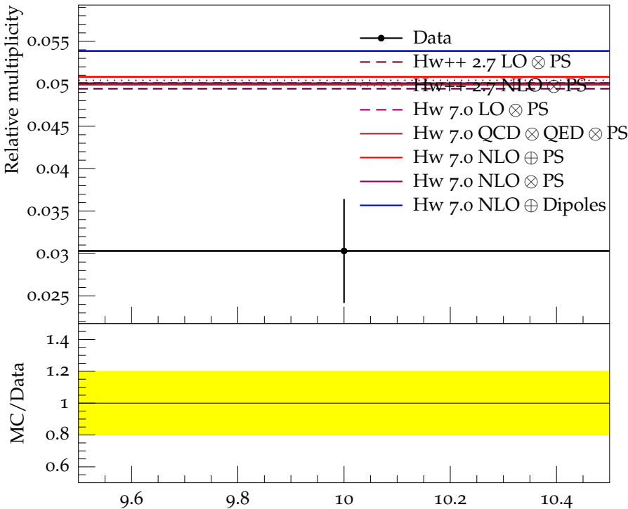
Ratio (w.r.t. \pi^\pm ) of mean \eta multiplicity
