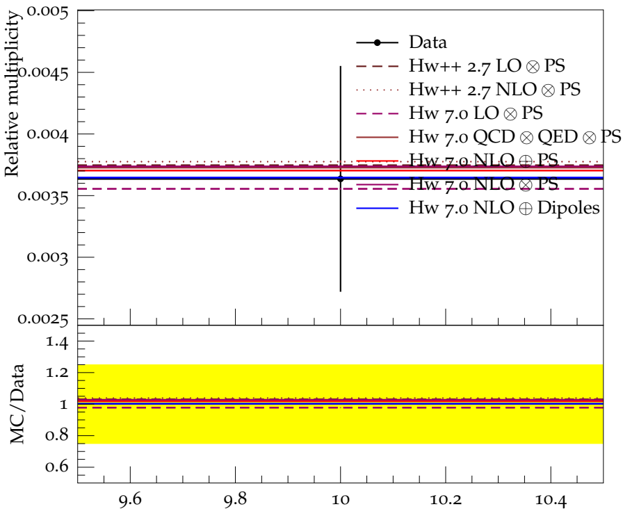
Ratio (w.r.t. \pi^\pm ) of mean f_0(980) multiplicity
