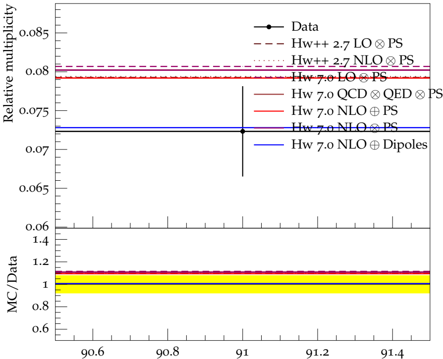
Ratio (w.r.t. \pi^\pm ) of mean \rho^0(770) multiplicity
