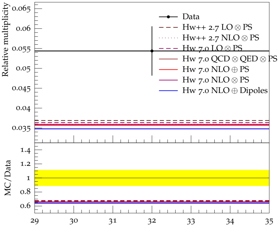
Ratio (w.r.t. \pi^\pm ) of mean K^{*0}(892) multiplicity
