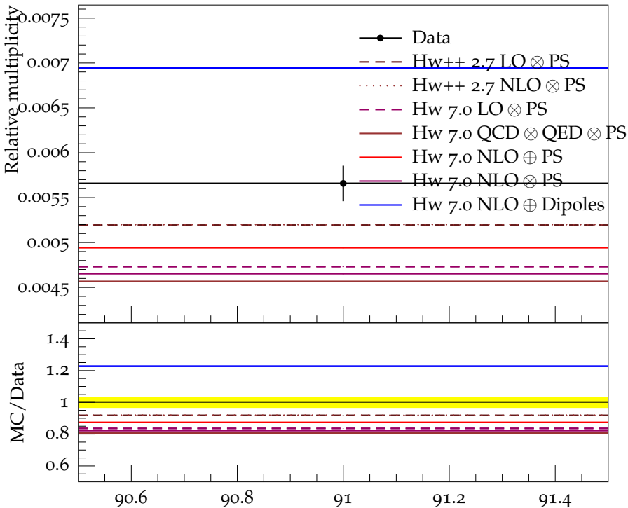
Ratio (w.r.t. \pi^\pm ) of mean \phi(1020) multiplicity
