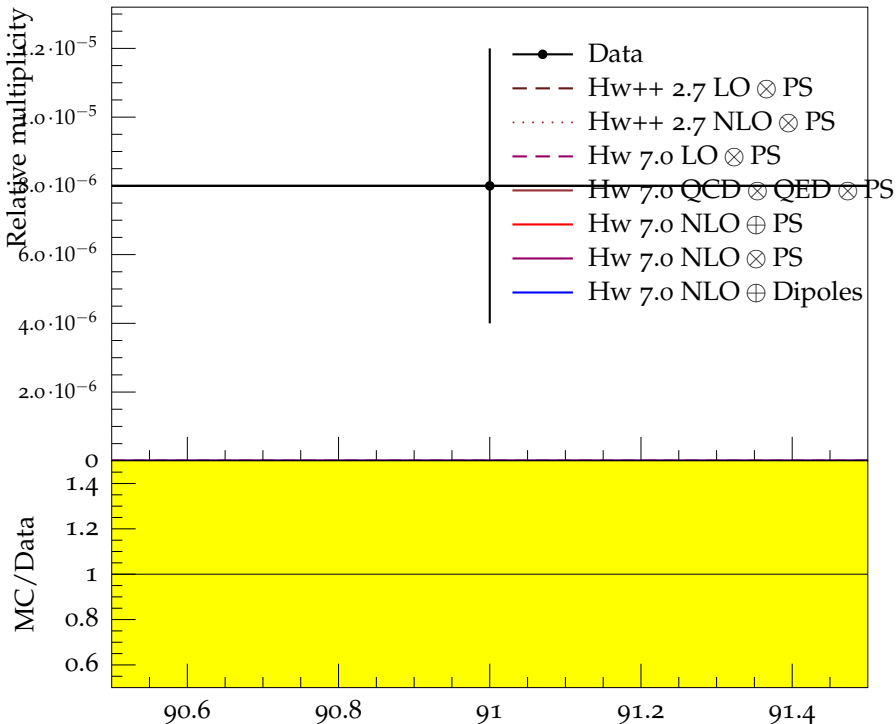
Ratio (w.r.t. \pi^\pm ) of mean Y(1S) multiplicity
