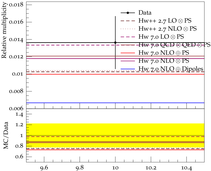
Ratio (w.r.t. \pi^\pm ) of mean f_2(1270) multiplicity
