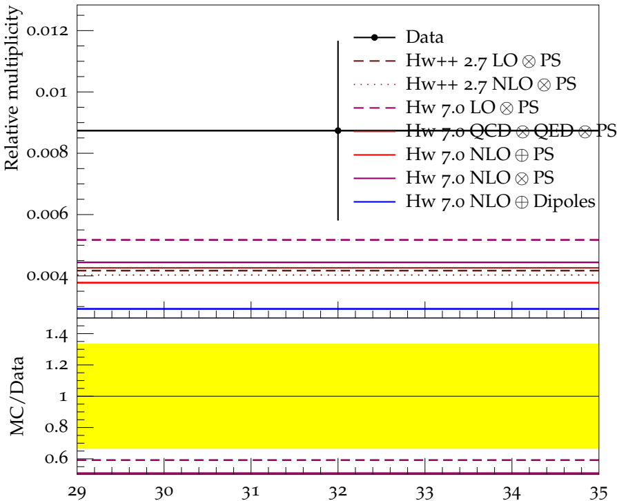
Ratio (w.r.t. \pi^\pm ) of mean K_2^{*+} (1430) multiplicity
