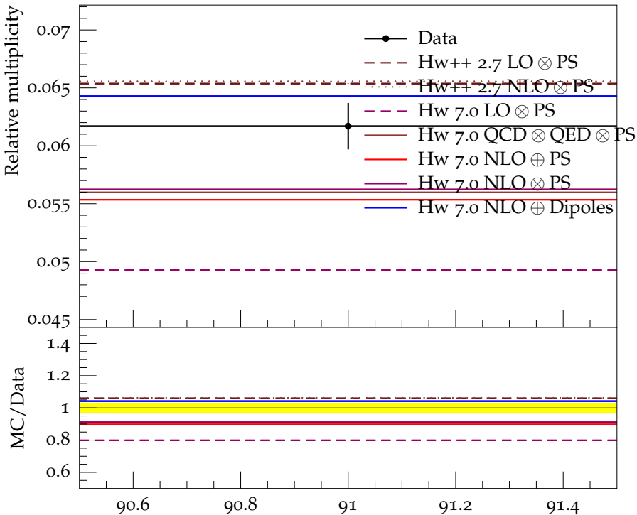
Ratio (w.r.t. \pi^\pm ) of mean p multiplicity
