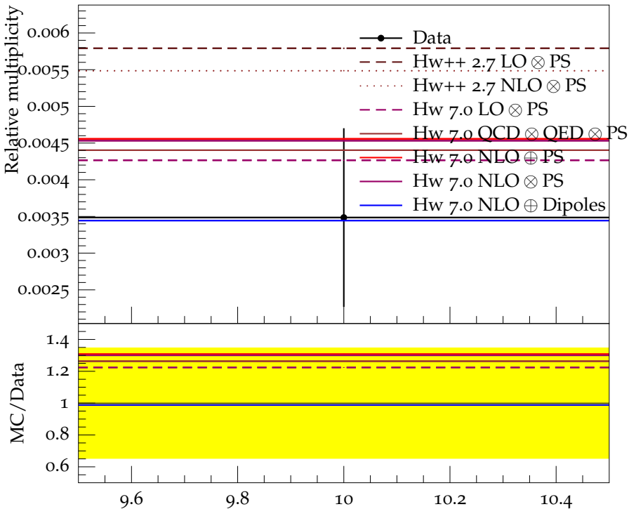
Ratio (w.r.t. \pi^\pm ) of mean \Sigma^0 multiplicity
