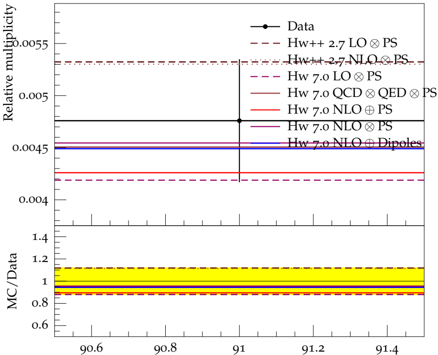
Ratio (w.r.t. \pi^\pm ) of mean \Sigma^- multiplicity
