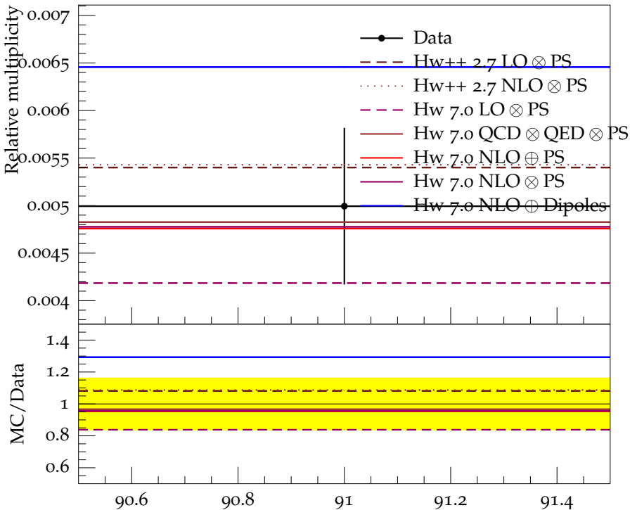
Ratio (w.r.t. \pi^\pm ) of mean \Delta^{++}(1232) multiplicity
