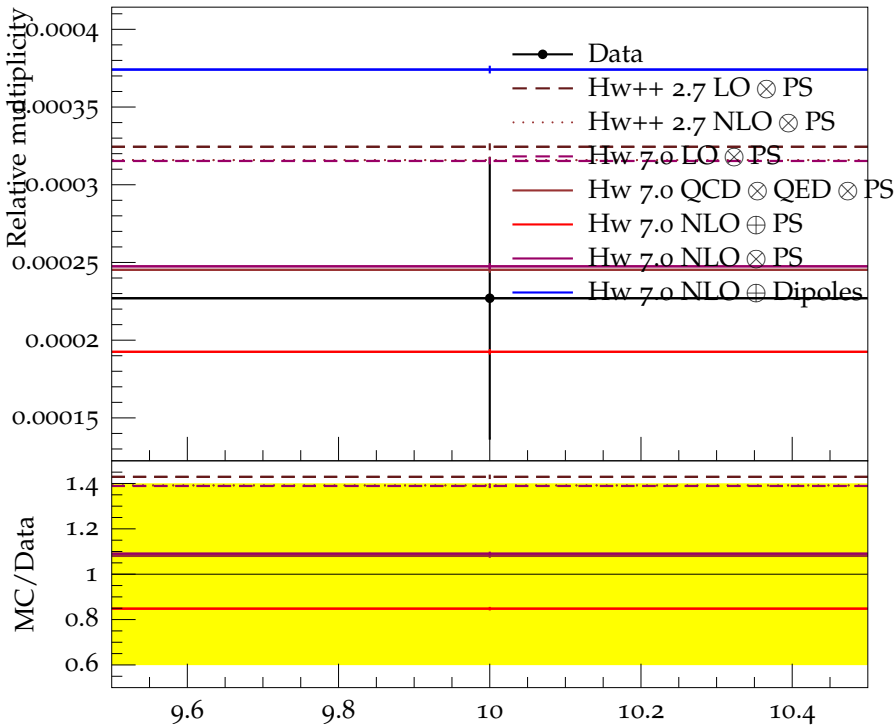
Ratio (w.r.t. \pi^\pm ) of mean \Xi^0(1530) multiplicity
