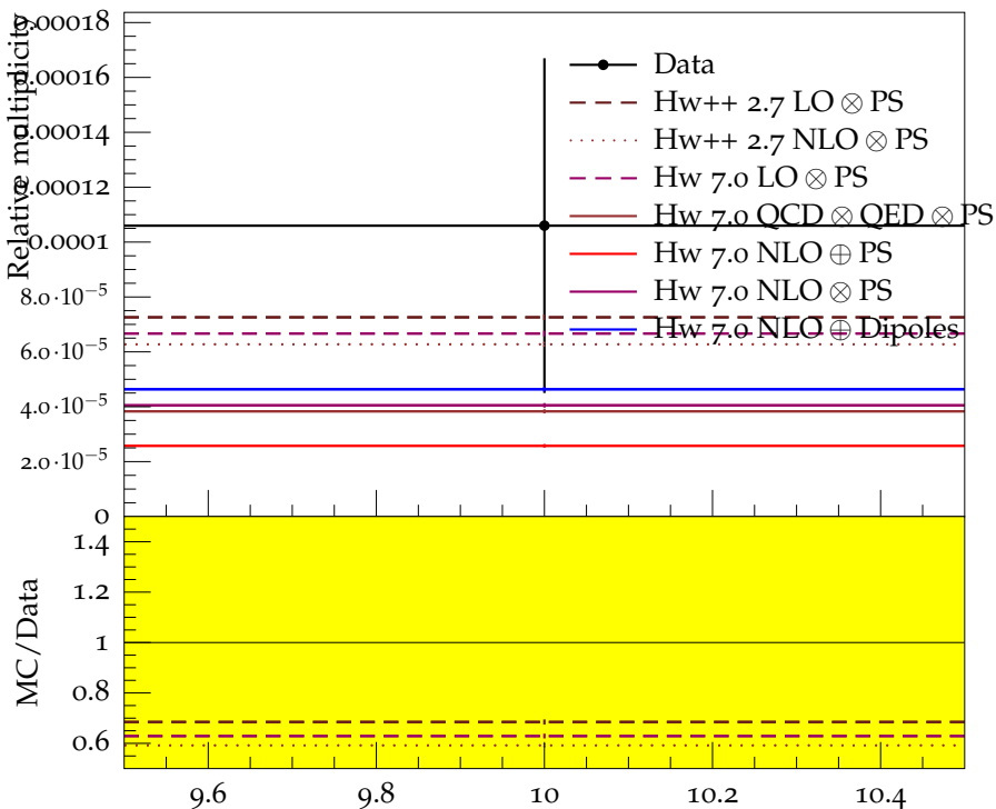
Ratio (w.r.t. \pi^\pm ) of mean \Omega^- multiplicity
