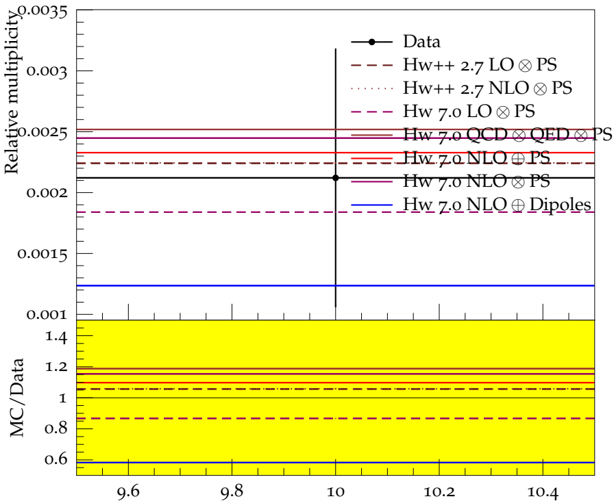
Ratio (w.r.t. \pi^\pm ) of mean \Sigma_c^{++} , \Sigma_c^0 multiplicity
